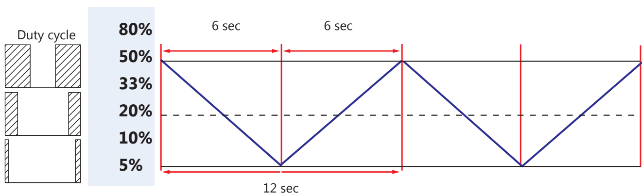
Figure 13: Duty cycle modulation (example of modulation at a selected duty cycle of 50%)
